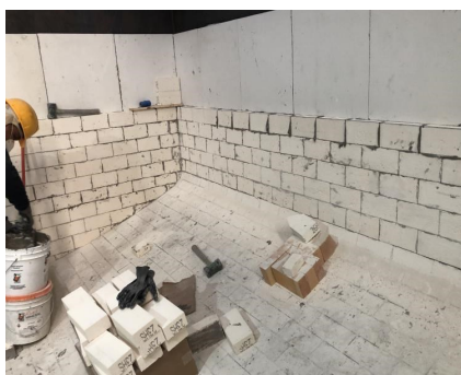
Insulating Fire Brick using BRIKSET
